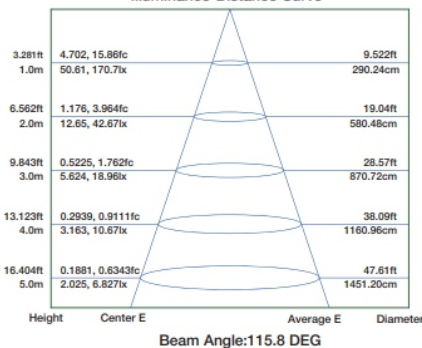
Illuminance-Distance Curve
